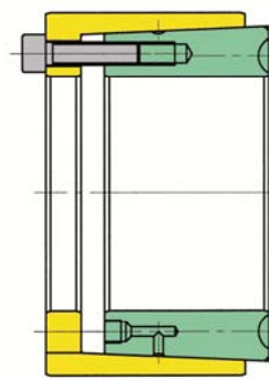
BIKON-Hydropress HPS
