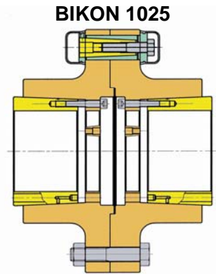
BIKON FKHS
